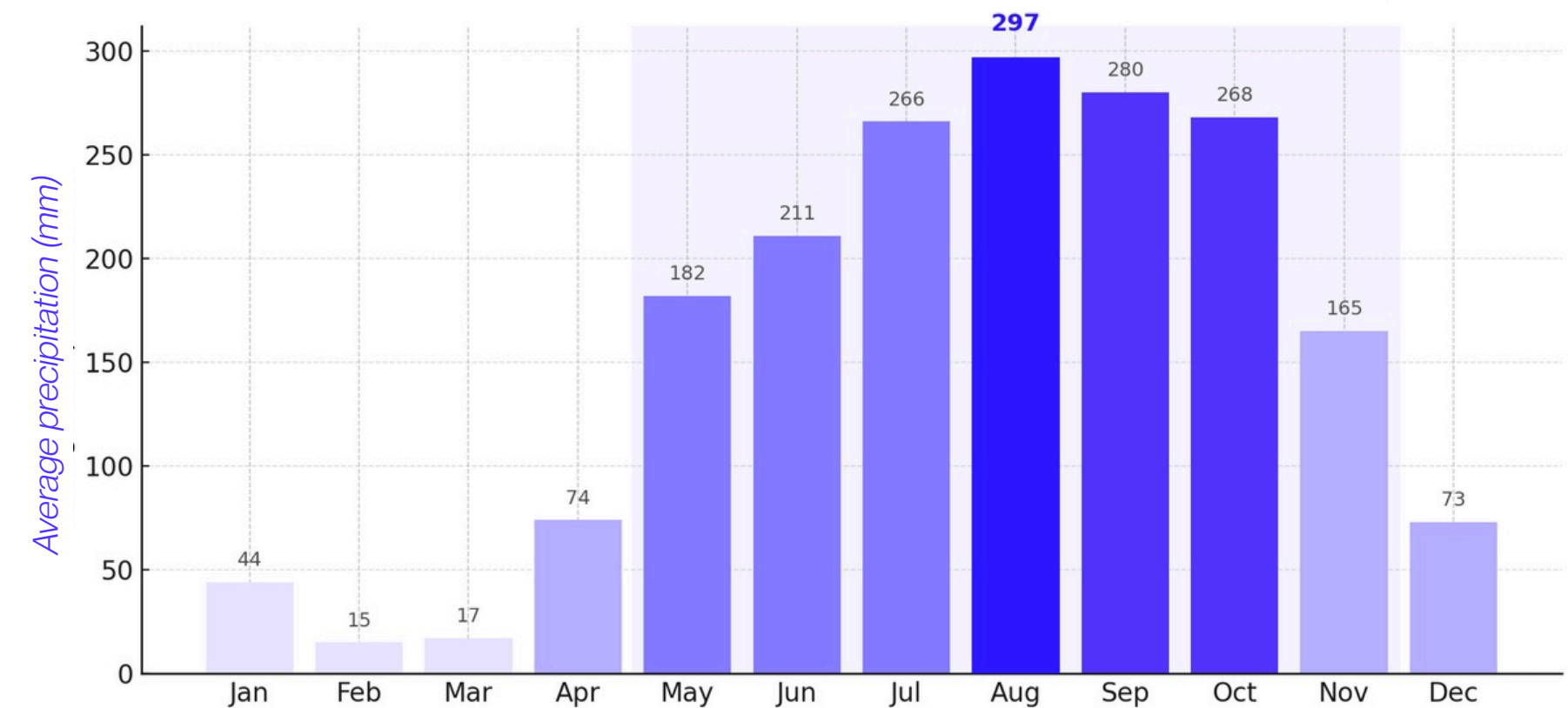
Monthly rainfall (mm) in Ho Chi Minh city (from 2017-2022)
