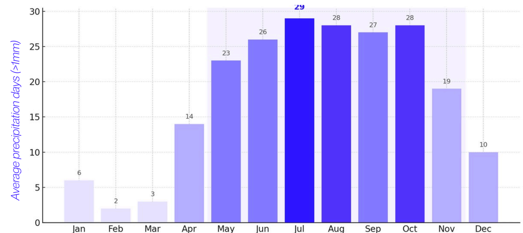
Average rainy days per month in Ho Chi Minh city (from 2017-2022)
